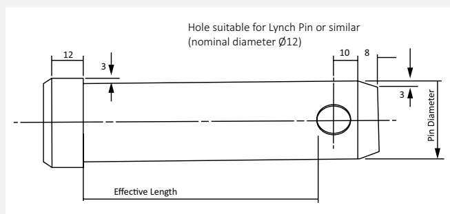
Figure 14.6 Typical pin design
