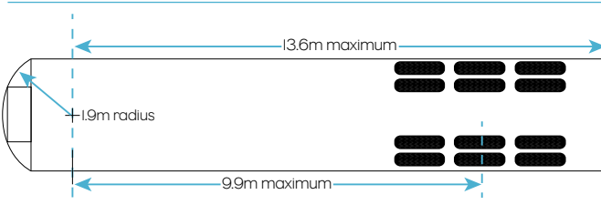
Figure 16.2 Refrigerated trailer
