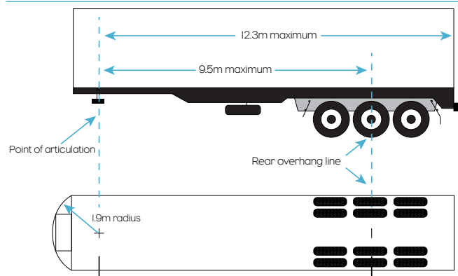
Figure 16.2 Refrigerated trailer
